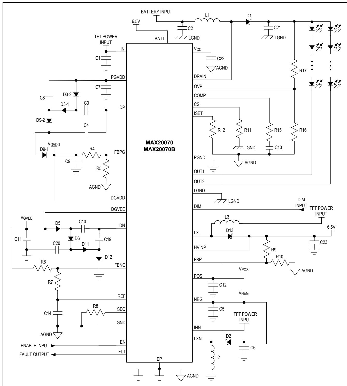
Figure 3. Simplified Operating Circuit for Coldcrank Below 4.5V
